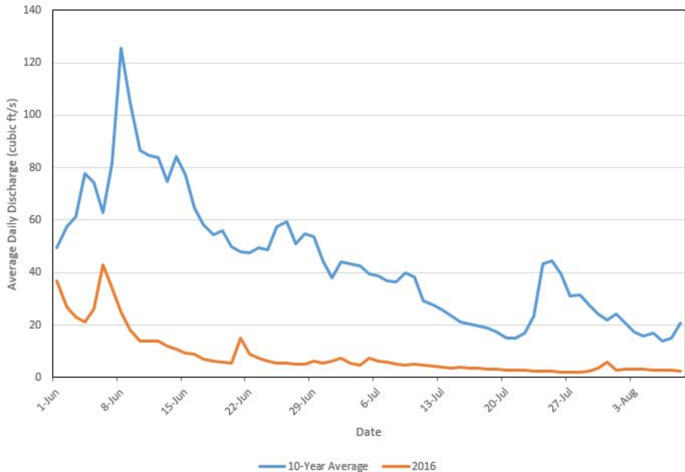
Average Daily Discharge, USGS Stream Gauge 1105000
